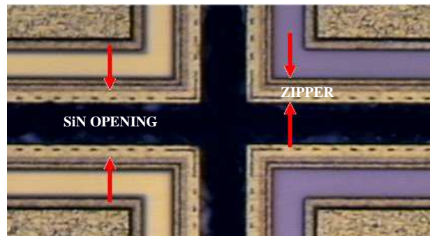
Figure 1. SiN Opening in Streets and on Part of Zippers
