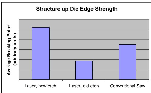
Figure 5. Impact of post laser dice etch on die edge strength
