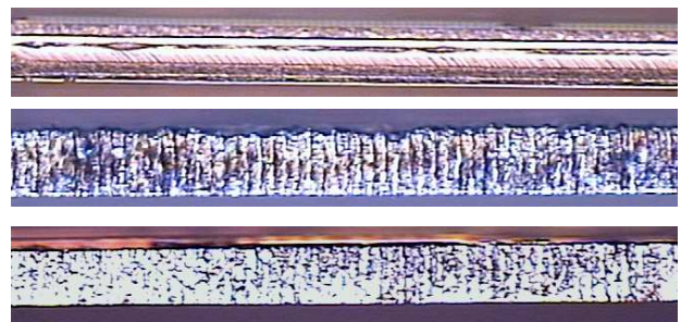
Figure 4. Die edge images typical for saw (top), laser diced with recast (center), laser diced after etch to remove recast (bottom)
