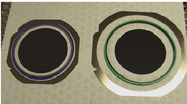
Figure 3. 6" wafers shown with original hoop and saw frame (Left) and current hoop and saw frame (Right)
