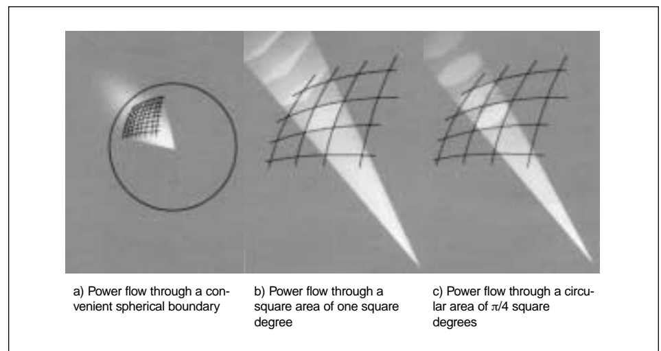
Figure 3. Simplified assumptions as to the shape of the radiated power yield approximate calculations of directive gain.
