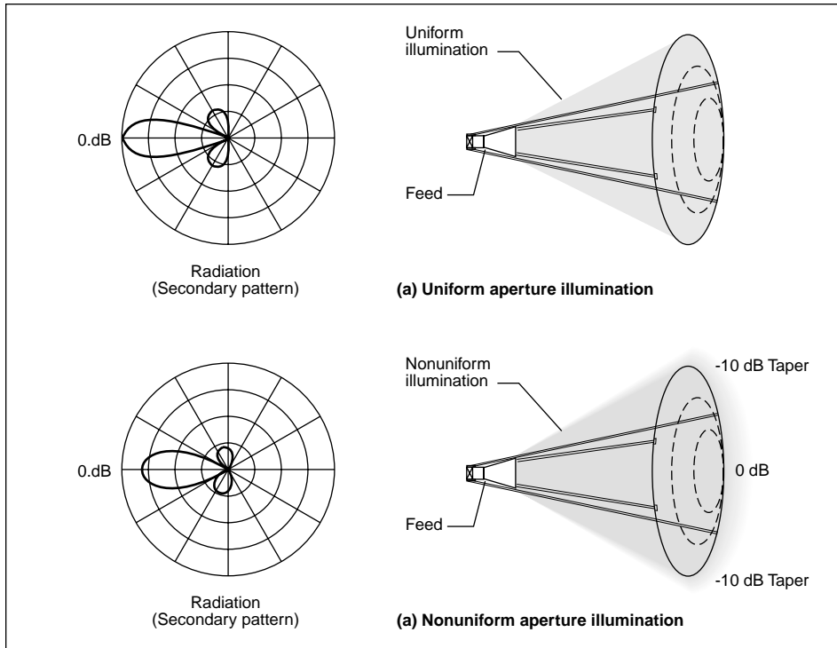
Figure 5. Field distributions, and radiation patterns produced, when a parabolic reflector's aperture is uniformly and nonuniformly illuminated.
