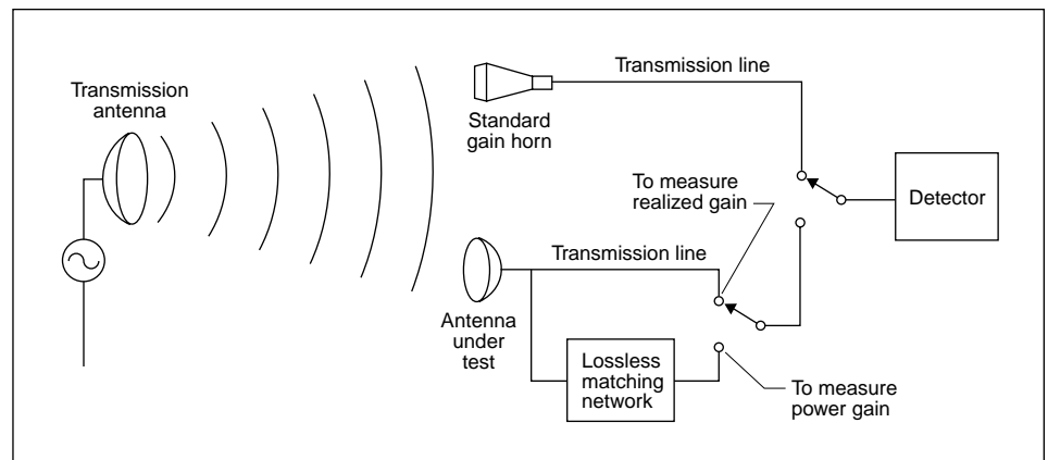
Figure 6. Power gain and realized gain measurements.
