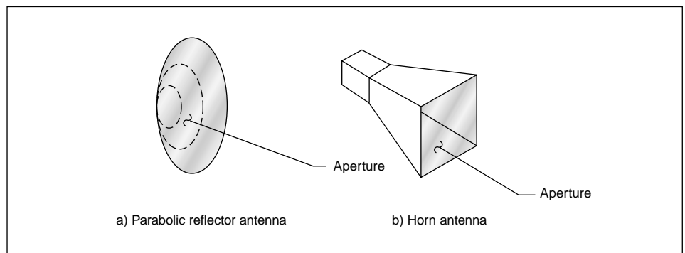
Figure 4. Physical apertures of parabolic reflector- and horn-type antennas.
