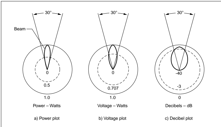
Figure 2. Equivalent half-power beamwidth representations of an antenna's radiation pattern.
