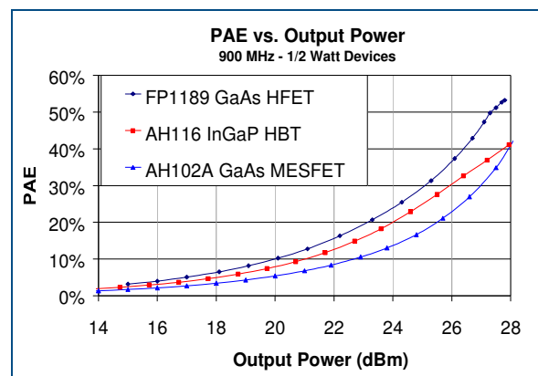
Figure 12. PAE vs. Output Power Plot (½-Watt devices)
