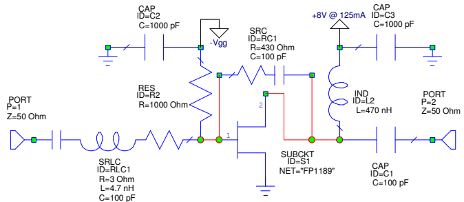
Figure 8. 130 – 900 MHz FP1189 Reference Design
