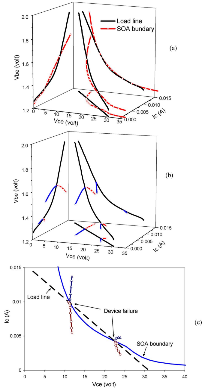
Fig. 6. (a) Three dimensional plot of a load line that interests the SOA boundary in two places. (b) Three dimensional plot of the I-V characteristics of the two fingers when the load line crosses the SOA boundary. (c) Two-finger I-V characteristics in the I_c-V_{ce} plane.
