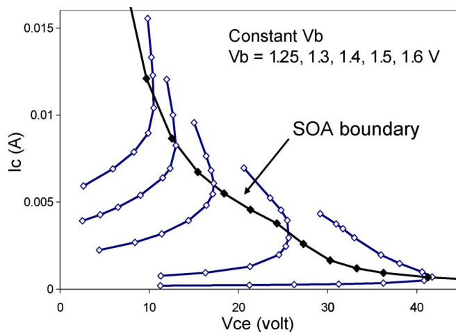
Fig. 3. Device I-V characteristics with various V_{be} inputs. The bend-over points are the places that the device becomes unstable. Therefore, the connection of the bend-over points is the SOA boundary.
