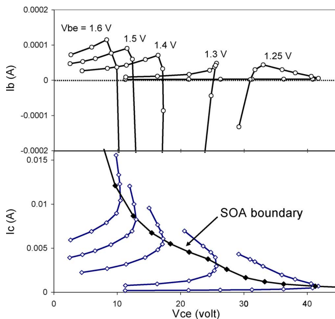
Fig. 4. Base-currents of the device curves shown in Fig. 3. The base-current reversal is due to the avalanche current being injected back into the base, and it indicates the onset of the device instability when the KIB is the dominant failure mechanism.
