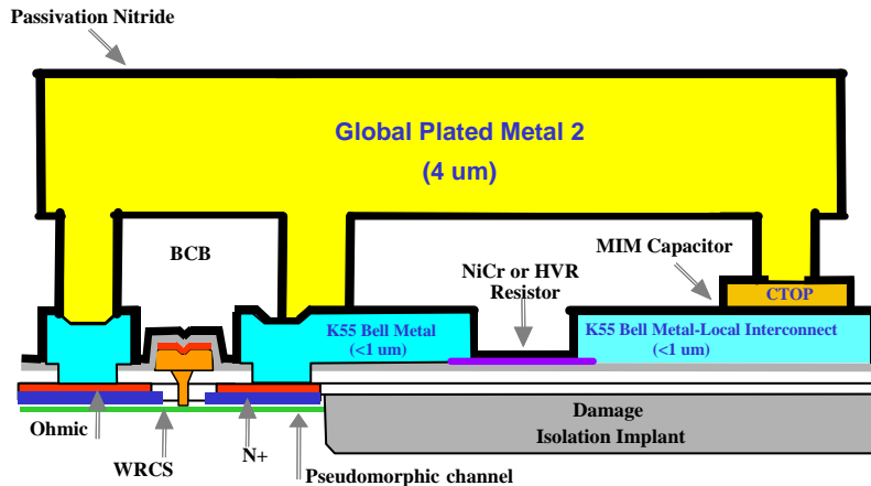
TQP15 Process Cross-Section
